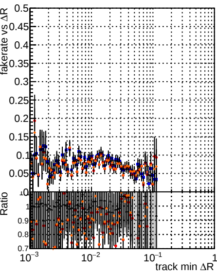
Fake rate vs \Delta R(\text{track, jet}) for base, trainOldFiles125_v2_prelimWPM_epoch4, and retrainOldFiles125_v2_prelimWPM_epoch4 models. Legend: DOM mkFile5 (blue squares), DOM mkFile6 (orange circles), OGDHighPt (black triangles).
