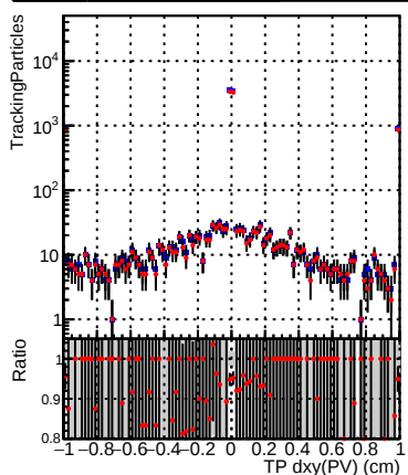
N of sim DQM_CKF_XiMinusPU_base DQM_CKF_XiMinusPU_retrainOldFiles125_v2_prelimWPM_epoch4
