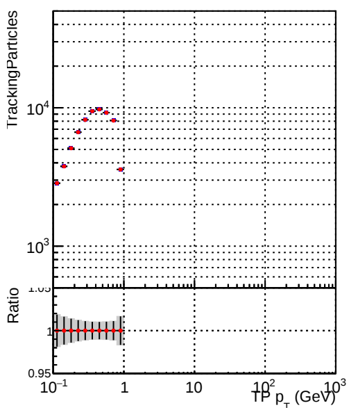
Legend: DQM_CKF_XiMinusPU_base (blue squares), DQM_CKF_XiMinusPU_retrainOldFiles125_v2_prelimWPM_epoch4 (red circles)
