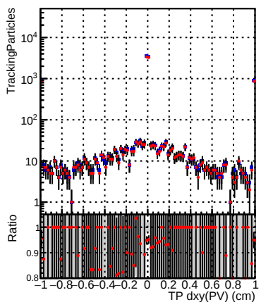
N of sim DQM_CKF_XiMinusPU_retrainOldFiles125_v2_prelimWPM_epoch4
