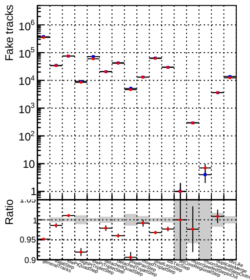
Number —●— DQM_CKF_XiMinusPU_retrainOldFiles125_v2_prelimWPM_epoch4
