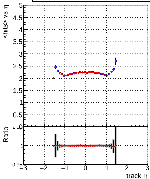
mean hits vs \eta — DQM_CKF_XiMinusPU_base — DQM_CKF_XiMinusPU_retrainOldFiles125_v2_prelimWPM_epoch4
