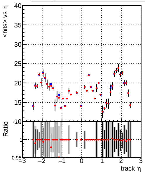
mean hits vs \eta Legend: DQM_CKF_XiMinusPU_base (blue line), DQM_CKF_XiMinusPU_retrainOldFiles125_v2_prelimWPM_epoch4 (red line)
