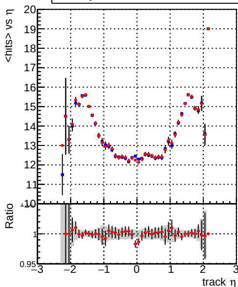
mean hits vs \eta — DQM_CKF_XiMinusPU_base — DQM_CKF_XiMinusPU_retrainOldFiles125_v2_prelimWPM_epoch4
