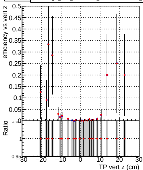
Efficiency vs. vert z — DQM_CKF_XiMinusPU_base — DQM_CKF_XiMinusPU_retrainOldFiles125_v2_prelimWPM_epoch4
