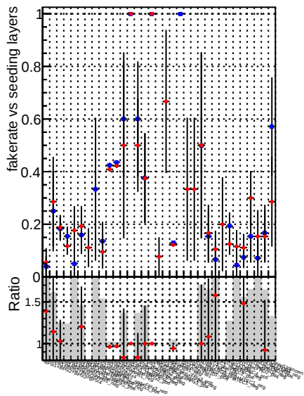
Fake rate vs. —•— DQM_CKF_XiMinusPU_base —•— DQM_CKF_XiMinusPU_retrainOldFiles125_v2_prelimWPM_epoch4
