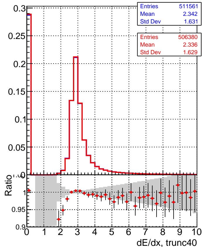
—■— DQM_CKF_XiMinusPU_base —●— DQM_CKF_XiMinusPU_retrainOldFiles125_v2_prelimWPM_epoch4
