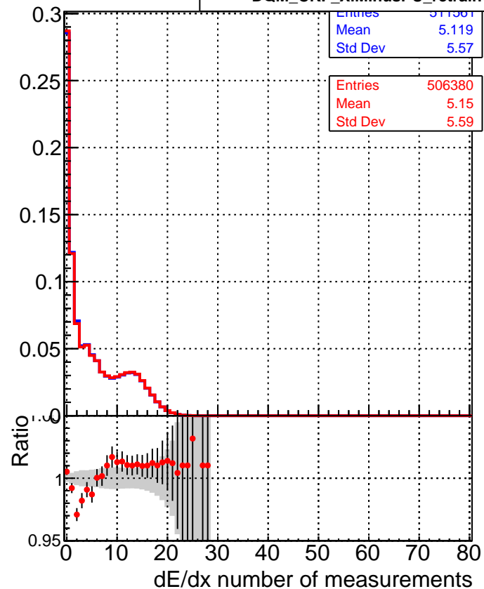
—■— DQM_CKF_XiMinusPU_base —●— DQM_CKF_XiMinusPU_retrainOldFiles125_v2_prelimWPM_epoch4
