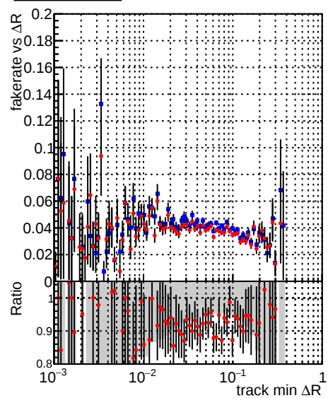
Fake rate vs \Delta R(\text{track, jet}) Legend: —•— DQM_CKF_XiMinusPU_base —•— DQM_CKF_XiMinusPU_retrainOldFiles125_v2_prelimWPM_epoch4
