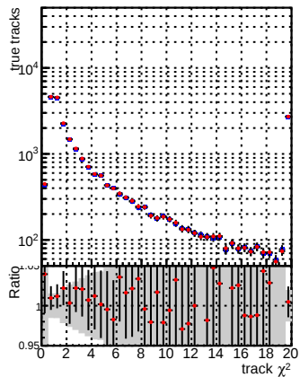
N of reco track vs. \chi^2 DQM_CKF_XiMinusPU_base DQM_CKF_XiMinusPU_retrainOldFiles125_v2_prelimWPM_epoch4
