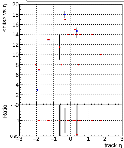
mean hits — DQM_CKF_XiMinusPU_base — DQM_CKF_XiMinusPU_retrainOldFiles125_v2_prelimWPM_epoch4
