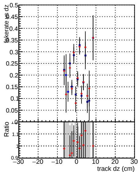
Fake rate vs dz Legend: Blue dots: DQM_CKF_XiMinusPU_base Red dots: DQM_CKF_XiMinusPU_retrainOldFiles125_v2_prelimWPM_epoch4
