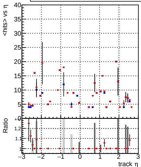
mean hit — DQM_CKF_XiMinusPU_base — DQM_CKF_XiMinusPU_retrainOldFiles125_v2_prelimWPM_epoch4
