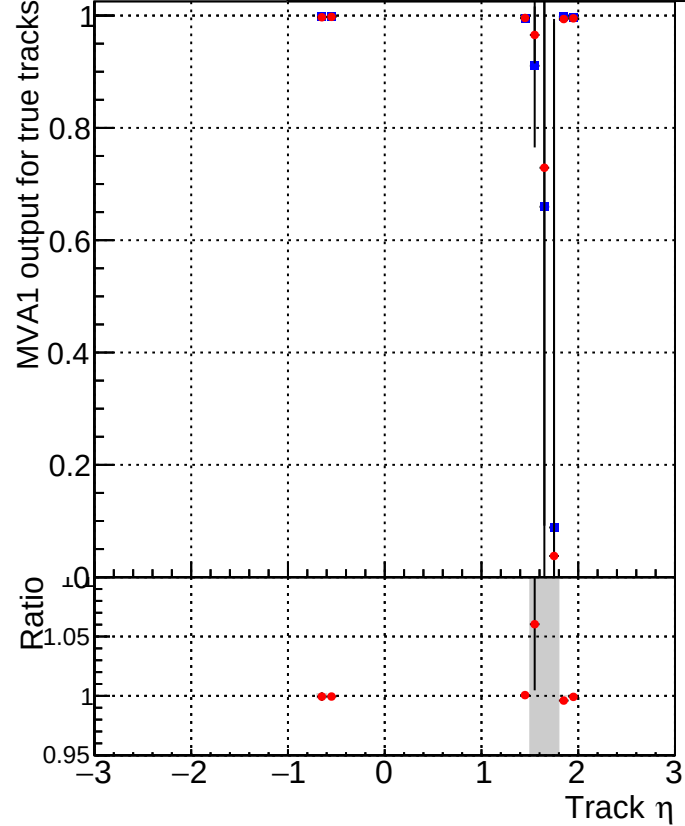
MVA1 of associated tracks (recoToSim) vs. track \eta Legend: DQM_CKF_XiMinusPU_base (blue squares) DQM_CKF_XiMinusPU_retrainOldFiles125_v2_prelimWPM_epoch4 (red circles)
