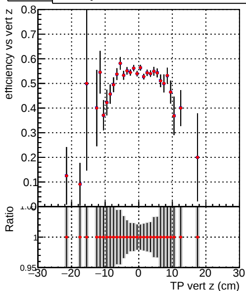
Efficiency vs. TP vert z — DQM_CKF_XiMinusPU_base — DQM_CKF_XiMinusPU_retrainOldFiles125_v2_prelimWPM_epoch4
