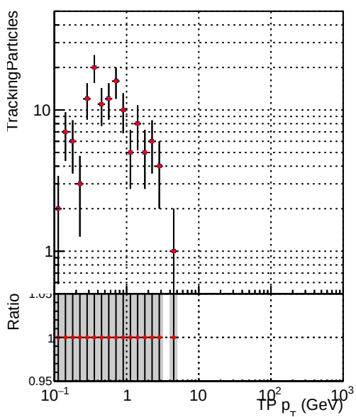
Legend: DQM_CKF_XiMinusPU_base (black line), DQM_CKF_XiMinusPU_retrainOldFiles125_v2_prelimWPM_epoch4 (red line)
