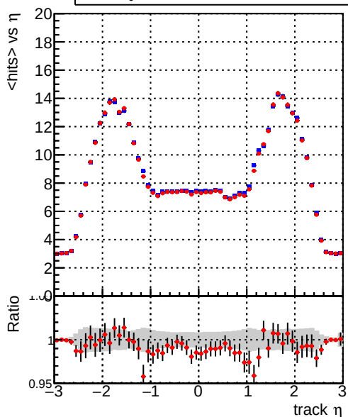
mean hits vs \eta Legend: DQM_CKF_XiMinusPU_base (blue line), DQM_CKF_XiMinusPU_retrainOldFiles125_v2_prelimWPM_epoch4 (red line)
