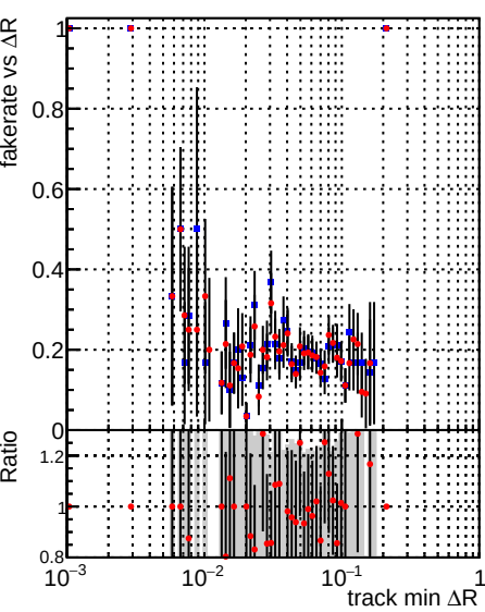
Legend: DQM_CKF_XiMinusPU_base DQM_CKF_XiMinusPU_retrainOldFiles125_v2_prelimWPM_epoch4
