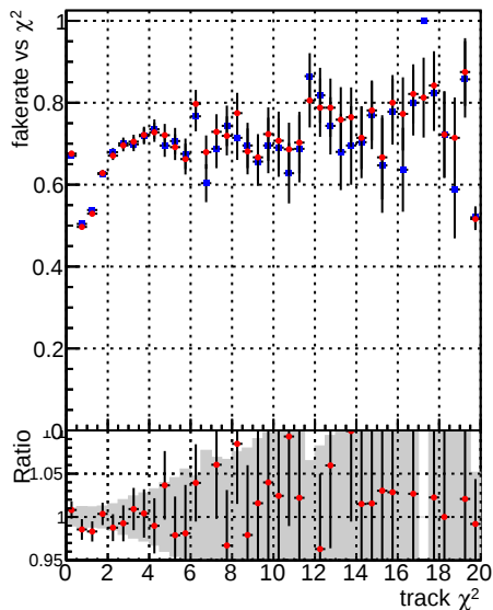
Fake rate vs. \chi^2 Legend: —•— DQM_CKF_XiMinusPU_base —•— DQM_CKF_XiMinusPU_retrainOldFiles125_v2_prelimWPM_epoch4
