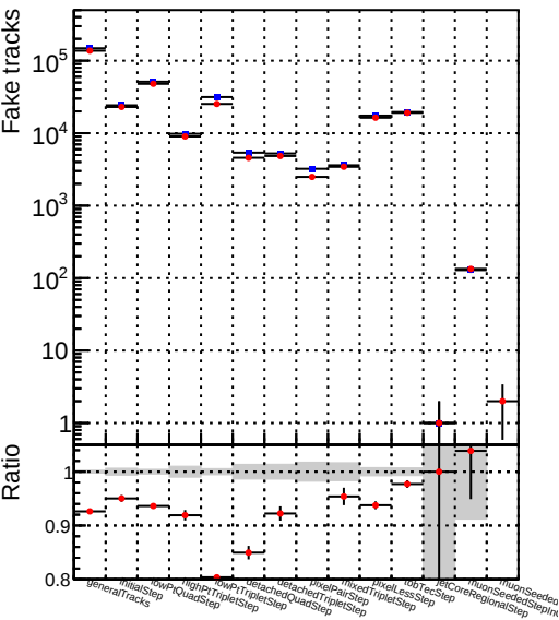
Number ● DQM_CKF_XiMinusPU_retrainOldFiles125_v2_prelimWPM_epoch3
