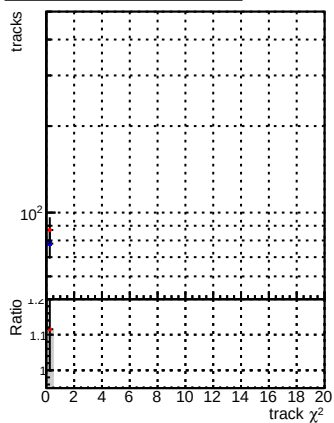
N of reco track vs. \chi^2 DQM_CKF_XiMinusPU_base DQM_CKF_XiMinusPU_retrainOldFiles125_v2_prelimWPM_epoch3
