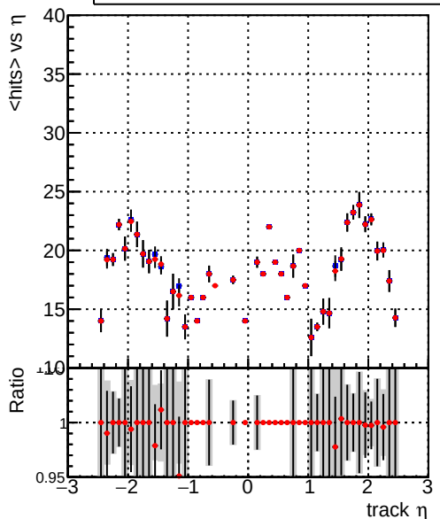
mean hits vs \eta Legend: DQM_CKF_XiMinusPU_base (blue line), DQM_CKF_XiMinusPU_retrainOldFiles125_v2_prelimWPM_epoch3 (red line)
