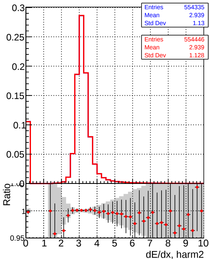
Legend: DQM_CKF_XiMinusPU_base (grey histogram) DQM_CKF_XiMinusPU_retrainOldFiles125_v2_prelimWPM_epoch3 (red line with markers)
