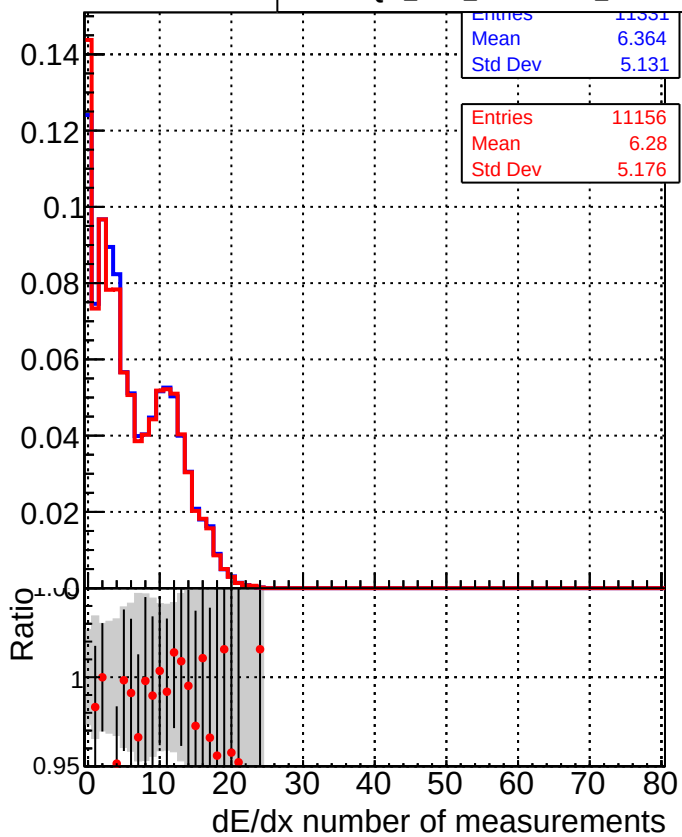
Legend: DQM_CKF_XiMinusPU_base (Blue line with squares) DQM_CKF_XiMinusPU_retrainOldFiles125_v2_prelimWPM_epoch3 (Red line with circles)
