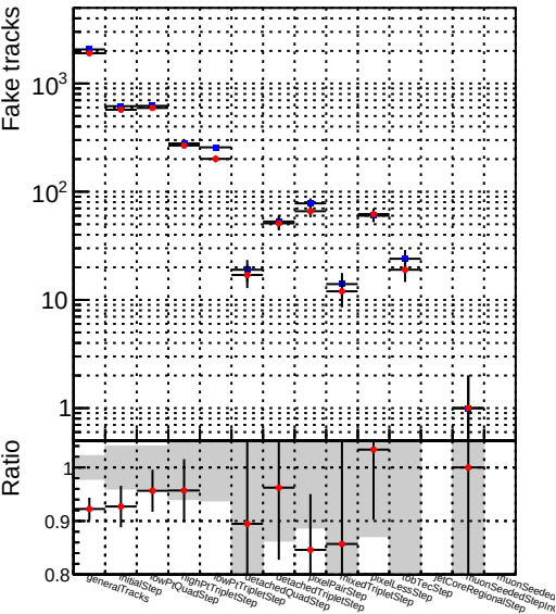
Numbe —●— DQM_CKF_XiMinusPU_retrainOldFiles125_v2_prelimWPM_epoch3
