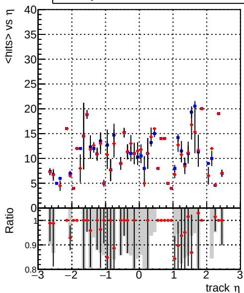
mean hits vs \eta Legend: DQM_CKF_XiMinusPU_base (blue line with circles), DQM_CKF_XiMinusPU_retrainOldFiles125_v2_prelimWPM_epoch3 (red line with circles)
