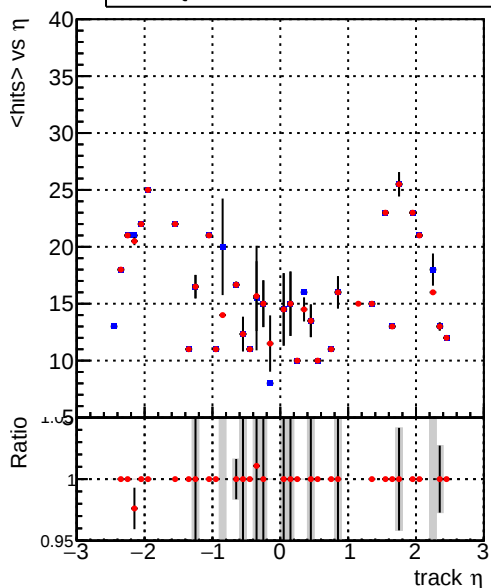
mean hit — DQM_CKF_XiMinusPU_base — DQM_CKF_XiMinusPU_retrainOldFiles125_v2_prelimWPM_epoch3
