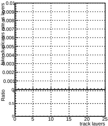
fake+duplicates
