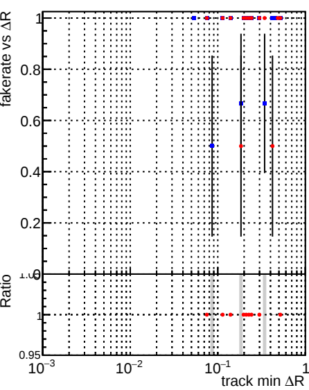
Legend: DQM_CKF_XiMinusPU_base DQM_CKF_XiMinusPU_retrainOldFiles125_v2_prelimWPM_epoch3
