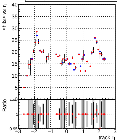
mean hits vs \eta Legend: DQM_CKF_XiMinusPU_base (blue line), DQM_CKF_XiMinusPU_retrainOldFiles125_v2_prelimWPM_epoch3 (red line)
