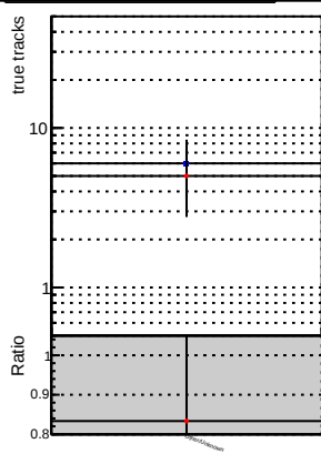
N of reco track vs. \chi^2 — DQM_CKF_XiMinusPU_base — DQM_CKF_XiMinusPU_retrainOldFiles125_v2_prelimWPM_epoch3
