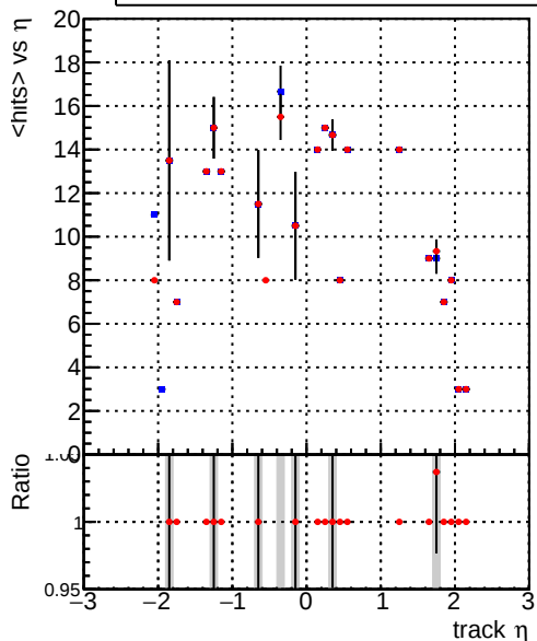
mean hit — DQM_CKF_XiMinusPU_base — DQM_CKF_XiMinusPU_retrainOldFiles125_v2_prelimWPM_epoch3
