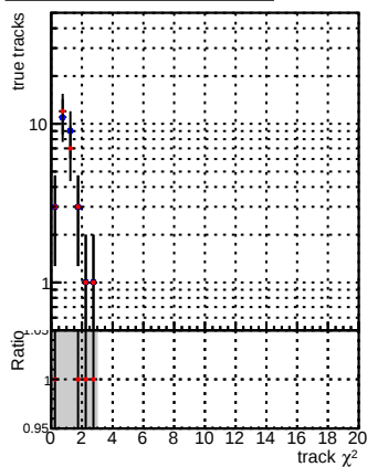
N of reco track vs. \chi^2 for DQM_CKF_XiMinusPU_base (blue) and DQM_CKF_XiMinusPU_retrainOldFiles125_v2_prelimWPM_epoch3 (red).
