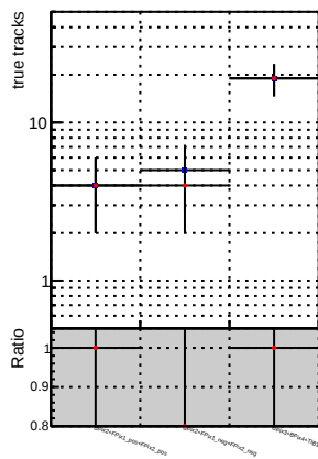
N of reco track vs. \chi^2 for DQM_CKF_XiMinusPU_base (blue) and DQM_CKF_XiMinusPU_retrainOldFiles125_v2_prelimWPM_epoch3 (red).
