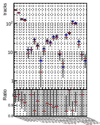
N of reco track vs. \chi^2 — DQM_CKF_XiMinusPU_base — DQM_CKF_XiMinusPU_retrainOldFiles125_v2_prelimWPM_epoch3
