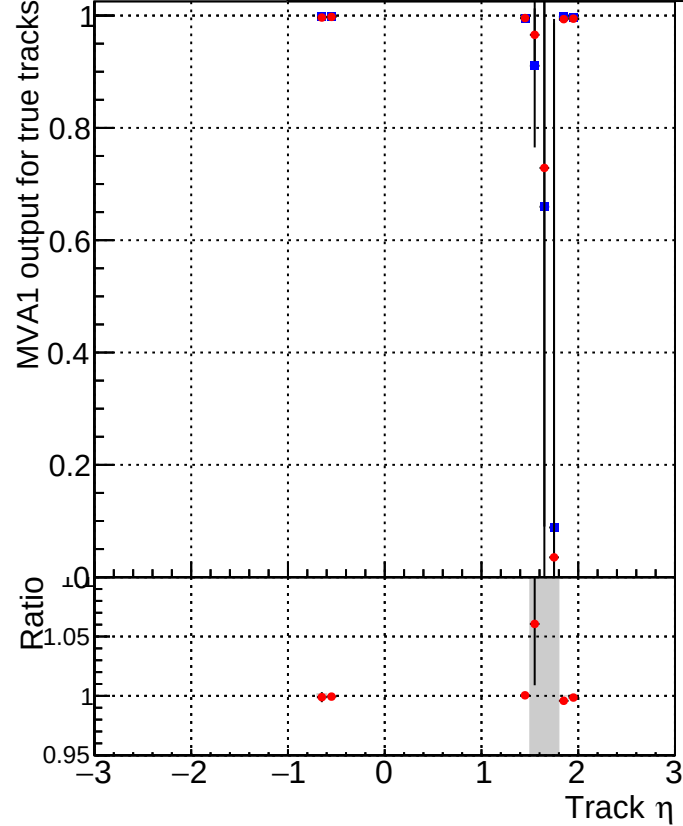
MVA1 of associated tracks (recoToSim) vs. track \eta Legend: DQM_CKF_XiMinusPU_base (blue squares) DQM_CKF_XiMinusPU_retrainOldFiles125_v2_prelimWPM_epoch3 (red circles)
