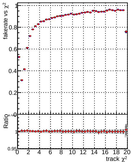
Fake rate vs. Legend: —●— DQM CKF XiMinusPU base —●— DQM CKF XiMinusPU_retrainOldFiles125_v2_prelimWPM_epoch3
