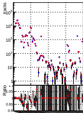
N of reco track vs. \chi^2 —●— DQM_CKF_XiMinusPU_base —●— DQM_CKF_XiMinusPU_retrainOldFiles125_v2_prelimWPM_epoch3
