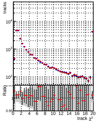
N of reco track vs. \chi^2 for DQM CKF XiMinusPU_base and DQM CKF XiMinusPU_retrainOldFiles125_v2_prelimWPM_epoch3
