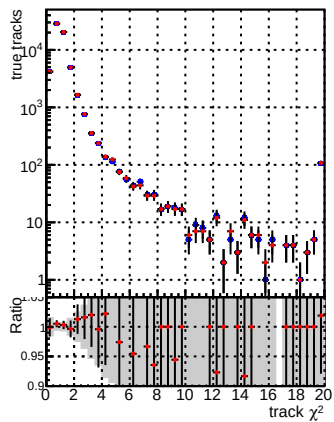
N of reco track vs. DQM CKF XiMinusPU_base DQM CKF XiMinusPU_retrainOldFiles125_v2_prelimWPM_epoch3
