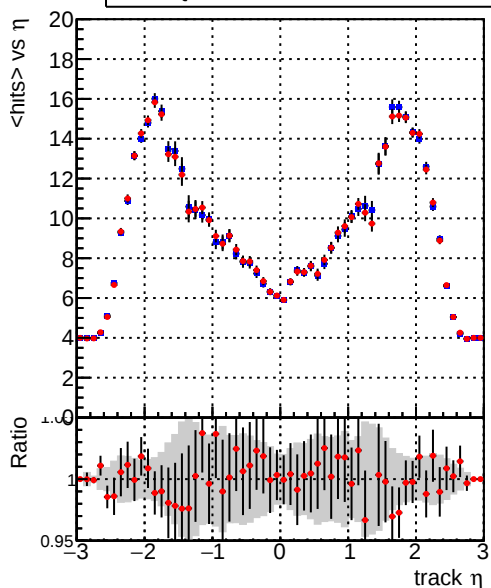
— DQM_CKF_XiMinusPU_base — DQM_CKF_XiMinusPU_retrainOldFiles125_v2_prelimWPM_epoch3 mean hits vs \eta
