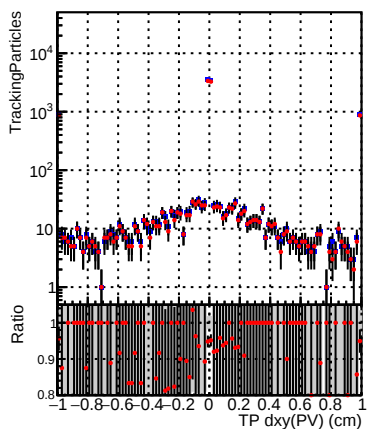
N of sim DQM_CKF_XiMinusPU_retrainOldFiles125_v2_prelimWPM_epoch2
