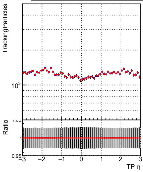
N of simulated tracks vs \eta Legend: \blacksquare DQM_CKF_XiMinusPU_base \bullet DQM_CKF_XiMinusPU_retrainOldFiles125_v2_prelimWPM_epoch2
