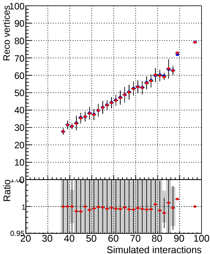
RecoVtx_vs_GenVtx
