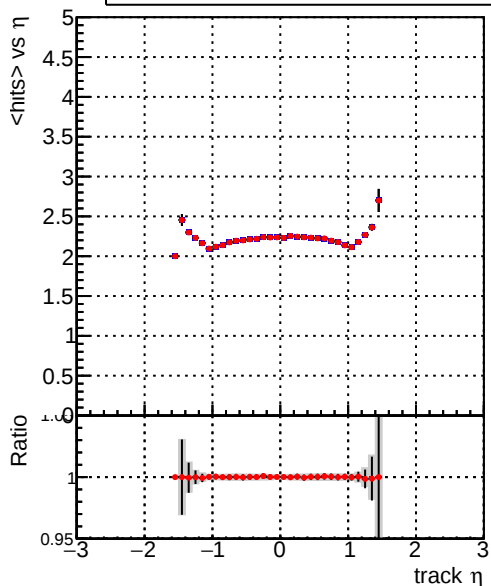
mean hits vs \eta — DQM_CKF_XiMinusPU_base — DQM_CKF_XiMinusPU_retrainOldFiles125_v2_prelimWPM_epoch2
