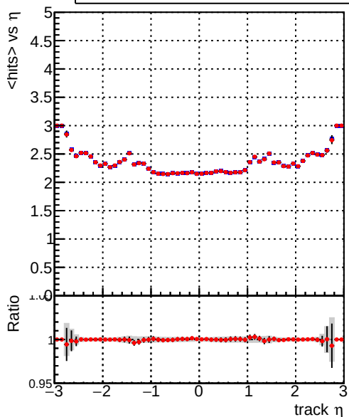
mean hits — DQM_CKF_XiMinusPU_base — DQM_CKF_XiMinusPU_retrainOldFiles125_v2_prelimWPM_epoch2
