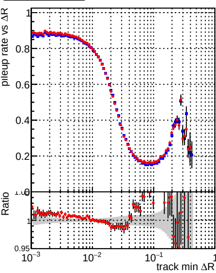
Legend: DQM_CKF_XiMinusPU_base (blue line with points), DQM_CKF_XiMinusPU_retrainOldFiles125_v2_prelimWPM_epoch2 (red line with points)
