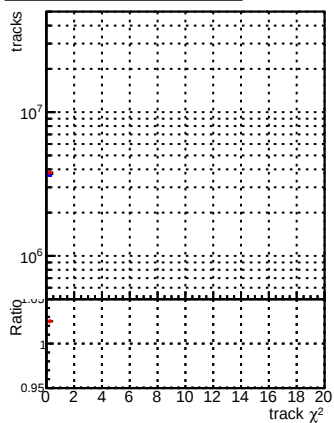
N of reco track vs. \chi^2 for different sets
